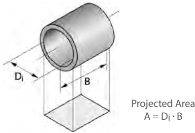
Fig. 6: Projected area for bearing
