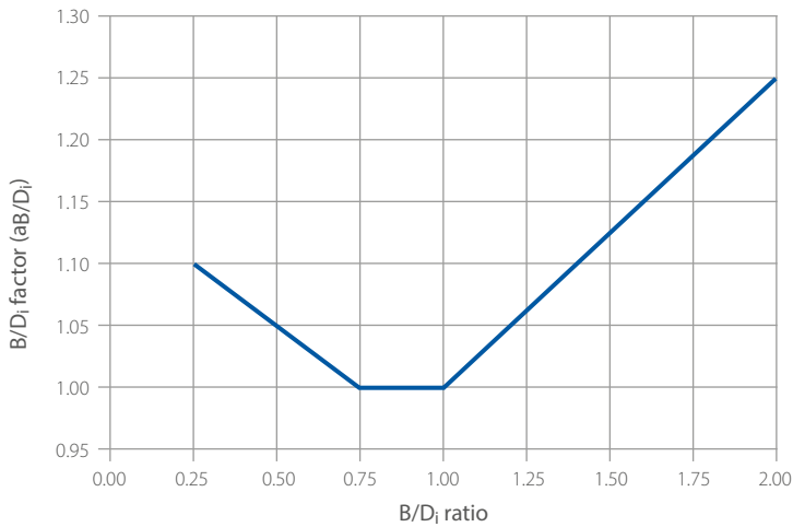
Fig. 8: B/D 1 factor (a B/D 1 )
