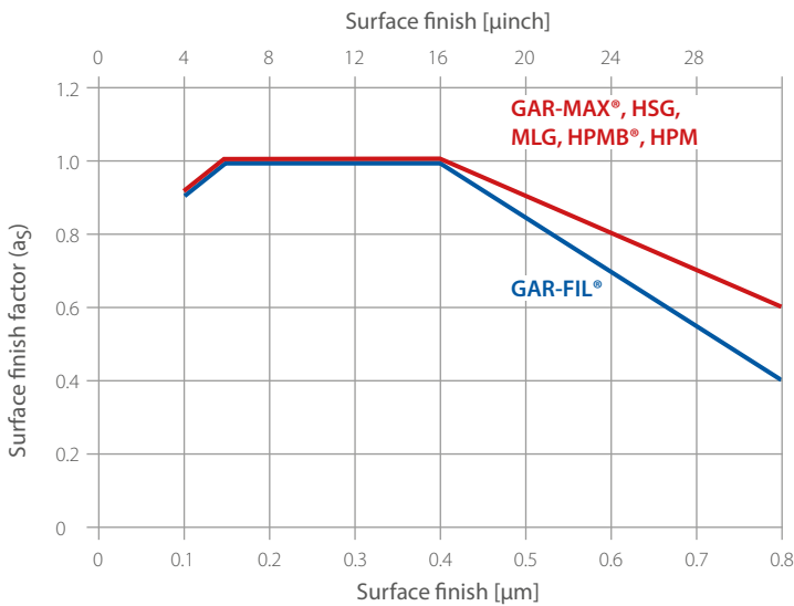
Fig. 12: Surface finish factor a_s
